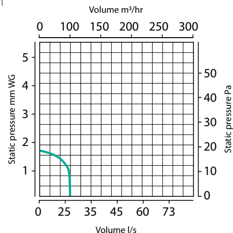
Fan Curves - Performance Graph Low Profile Units
